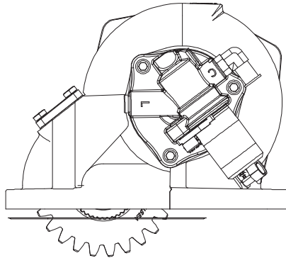
R = Valve Cap Rotated 120°
