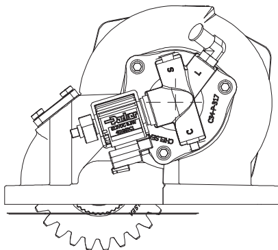
W = Wet Spline
