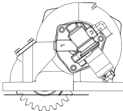
V = Valve Cap Rotated 120° w/ Wet Spline
