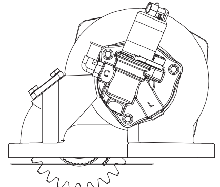
S = Valve Cap Rotated 240°
