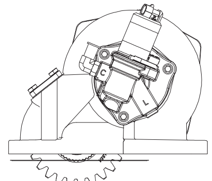
Y = Valve Cap Rotated 240° w/ Wet Spline
