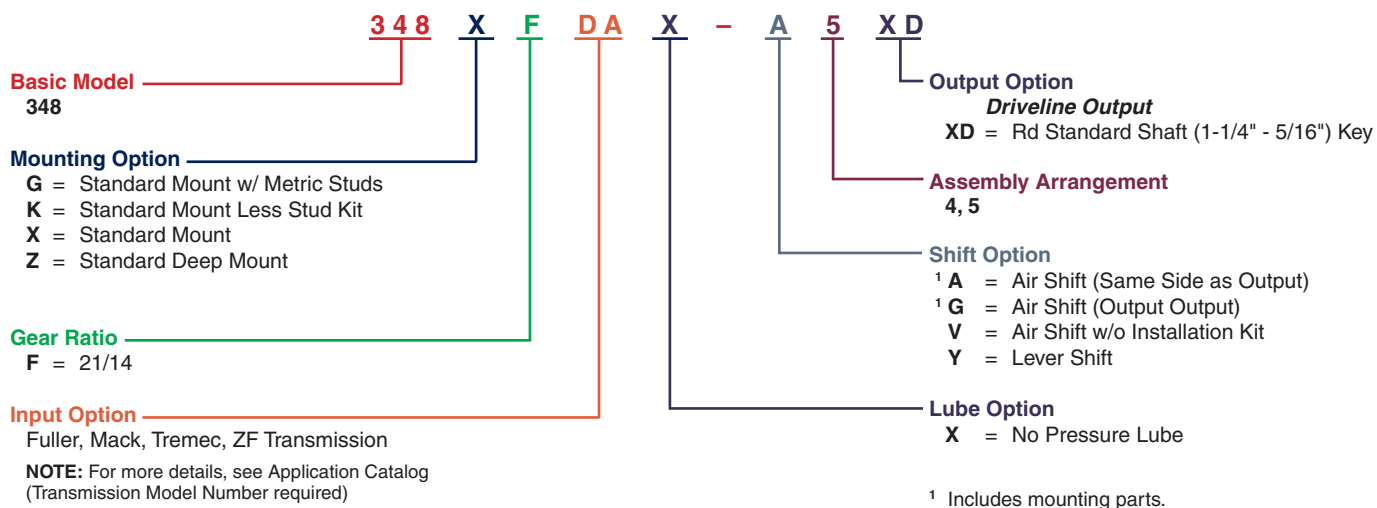
Shift Type A or G 5 Assembly Shown
