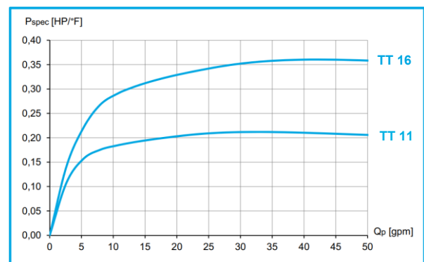
Specific cooling performance of Tanker Truck configurations (hydraulic fan drive)
